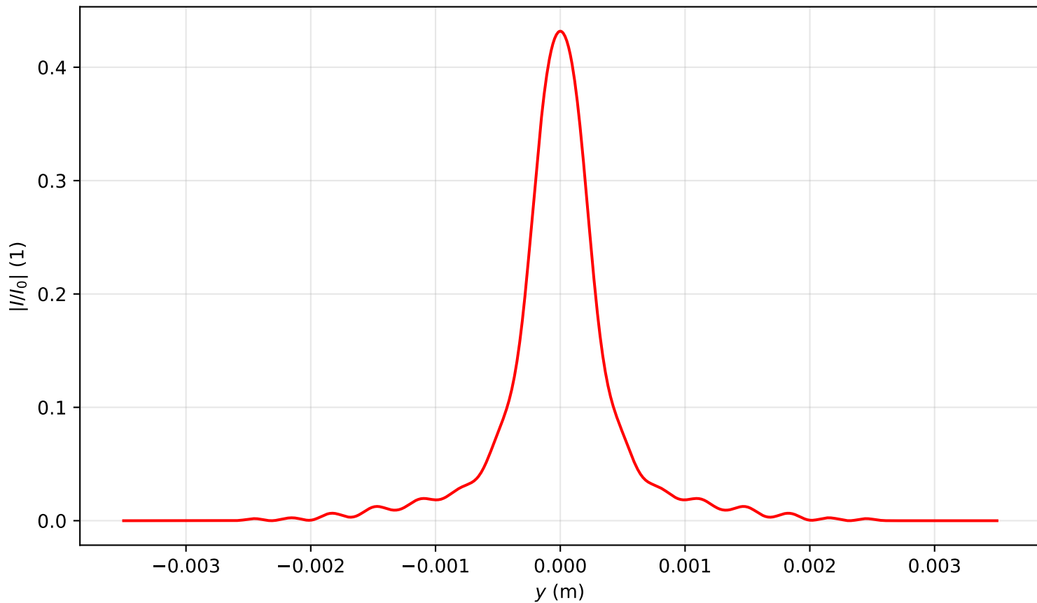
Intensity profile I(x=0, y, z=2.388)/I_0 , \text{Pin}=3.0\text{Pcr} , artificial time
